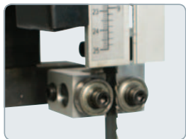
Ball Bearing Blade Guides BP-355
