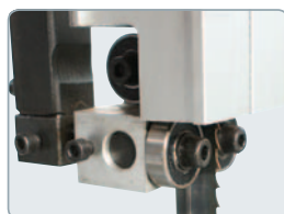
Ball Bearing Blade Guides BP-470
