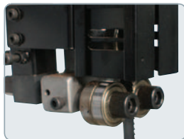
Ball Bearing Blade Guides BP-430 & BP-480
